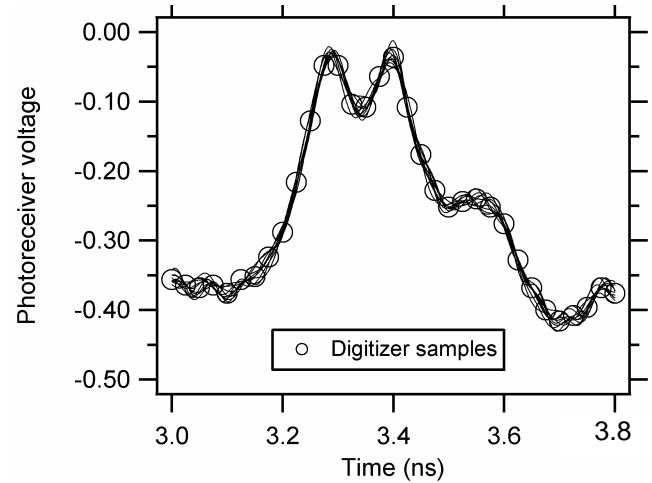
Fig. 10. Raw digitizer data (open circles) from the OMEGA experiment, together with ten of the one hundred Monte Carlo-simulated records used in the error estimation.
