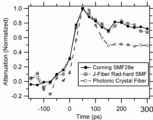
Fig. 7. Time response of the induced attenuation in the LINAC experiment for the three fibers tested using approximately 1 cm exposure length.
