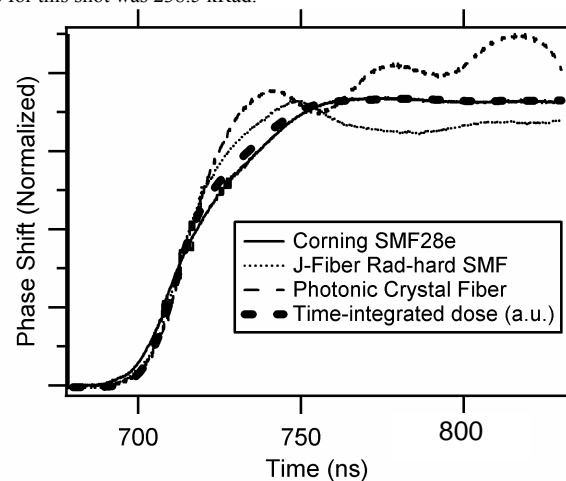
Fig. 4. Time response of the phase shift to a 30 ns wide electron pulse from the Febetron 705. The phase generally integrates the dose during exposure and recovers slowly for all three fibers tested.
