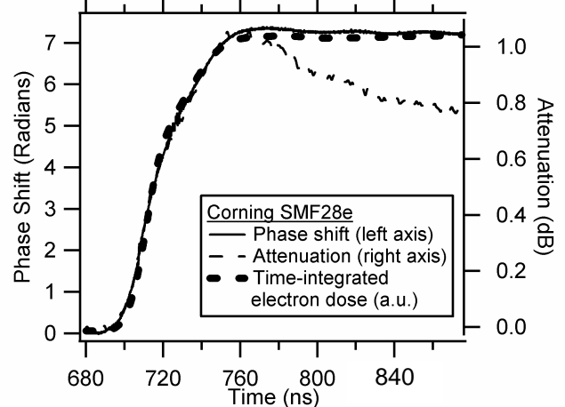
Fig. 3. Phase shift and attenuation of Corning SMF28e fiber during and immediately after exposure to the 30 ns pulse from the Febetron 705. Total dose for this shot was 238.5 kRad.
