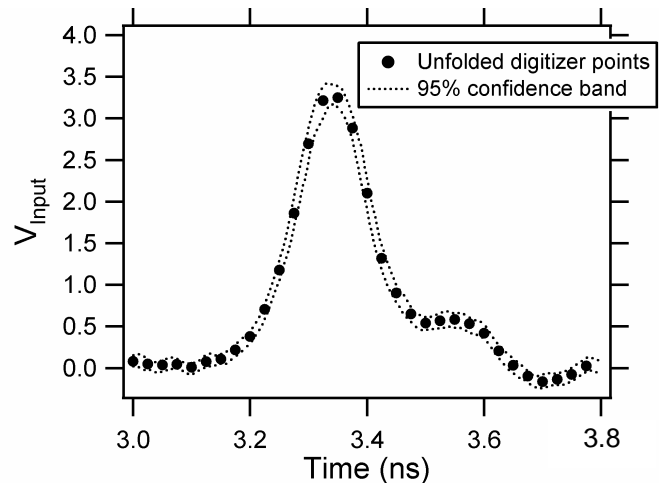
Fig. 11. Unfolded digitizer data (circles) from the OMEGA experiment, together with the 95% confidence bands from the Monte Carlo simulations.
