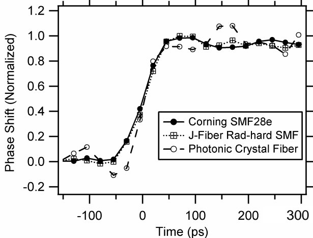
Fig. 8. Time response of the induced phase shift in the LINAC experiment for the three fibers tested using approximately 1 cm exposure length.
