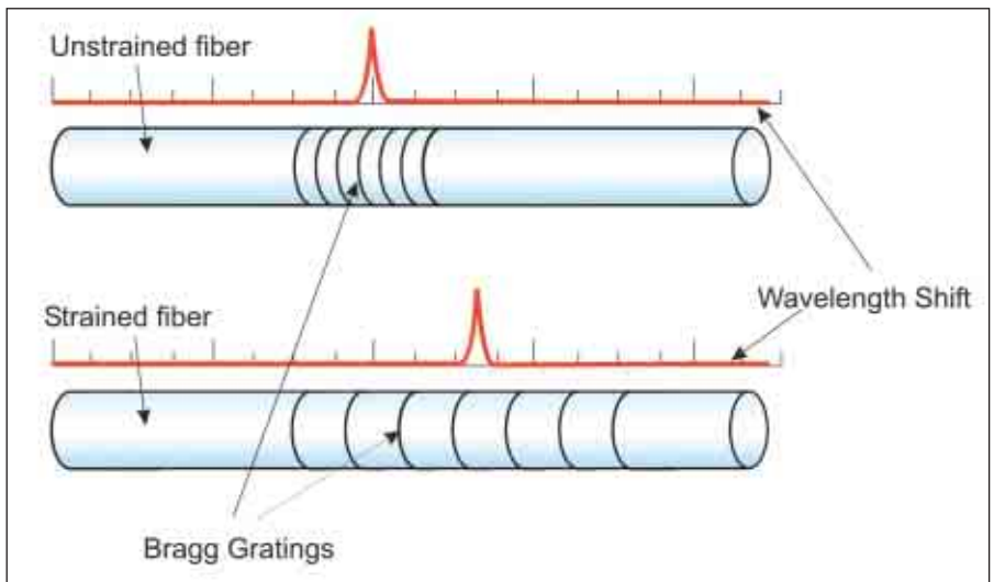
Figure 1. Fiber Bragg gratings are etched directly into the core of an optical fiber and, like a prism, disperse different colors (wavelengths) at different angles. Because these wavelengths are confined within a single-mode fiber, however, only a select few are able to propagate. The number and frequency of candidate wavelengths depends on the periodicity of the grating, which is sensitive to changes in temperature and fiber tension. Environmental changes at the grating location can therefore be detected as a change in wavelength.
