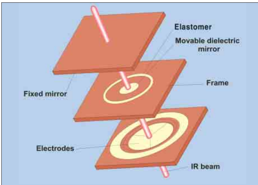
Figure 2. Many fiber-optic sensors probe specific wavelengths using a pair of microscopic mirrors—one fixed, the other movable—that vary their separation and establish a tunable spectral peak. One particular design incorporates elastomeric materials to support the mirrors, rendering a more stable and rugged configuration.
