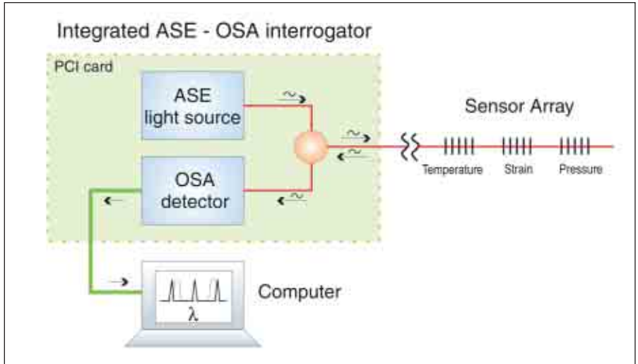
Figure 3. A simple, cost-effective fiber sensor configuration combines amplified-spontaneous emission (ASE) white light sources with optical spectrum analyzers (OSAs), all mounted on a single PCI card. Photons emitted by the fiber-based ASE source travel to the sensor gratings and return via fiber to the OSA detector. There, they are converted to electronic signals that a computer can analyze. Shifts in the optical signal indicate a perturbation at the sensing array.
