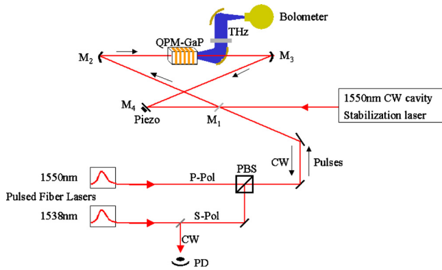
FIG. 2. (Color online) Experimental setup for cavity enhanced difference frequency THz generation. M_1 , cavity coupler; M_{2-3} , cavity curved mirrors; M_3 , dielectric mirror; PD, photodiode detector; S-POL, S polarization direction; P-POL, P-polarization direction; PBS, polarization beam splitter/combiner.
